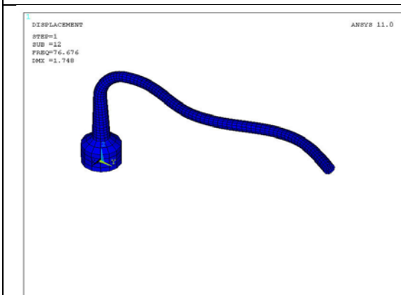
Figure 18 - Mode 7
