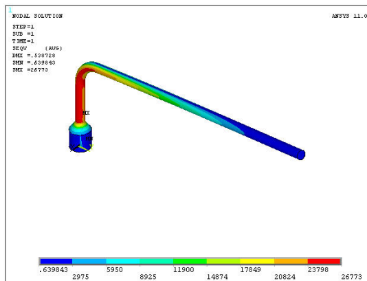
Figure 5 - 40 lb/ft Torque
