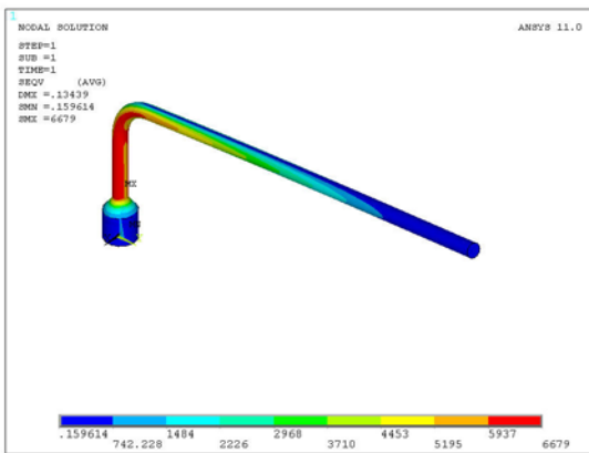
Figure 4 - 10 lb/ft Torque
