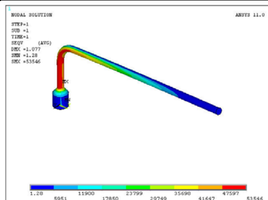
Figure 7 - 80 lb/ft Torque
