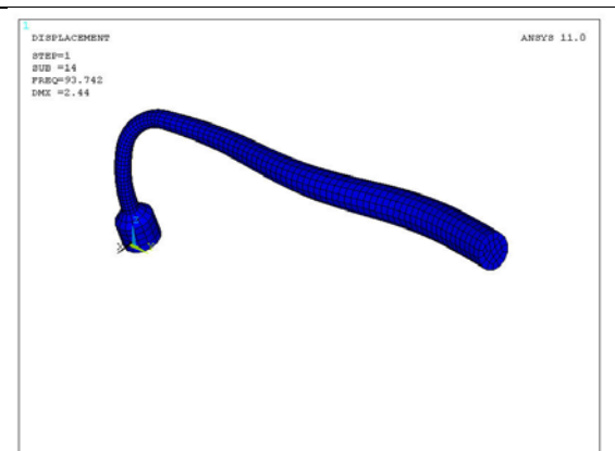
Figure 19 - Mode 8
