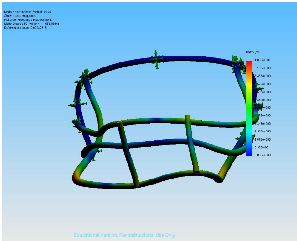
Figure 6: Frequency 10 at mesh size 0.1
