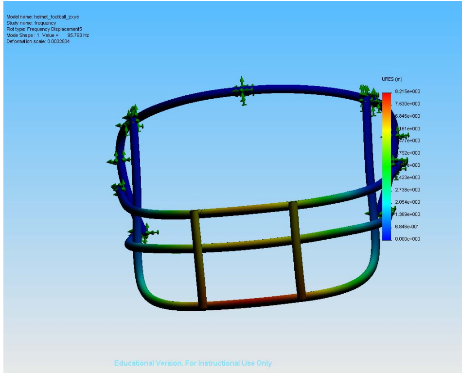
Figure 4: Frequency 1 at mesh size 0.1
