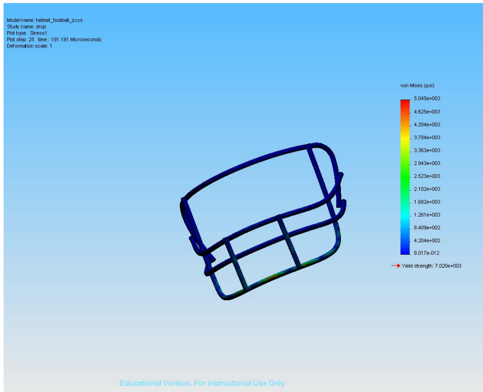
Figure 7: Stress plot after drop test
