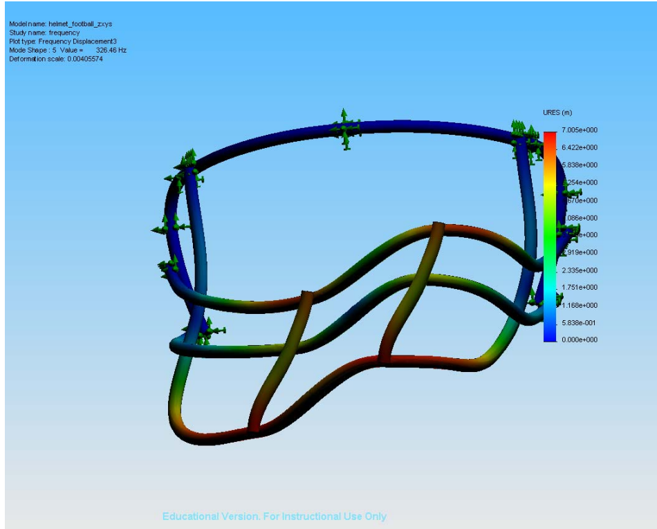
Figure 2: Modal shape & deformation at frequency 5
