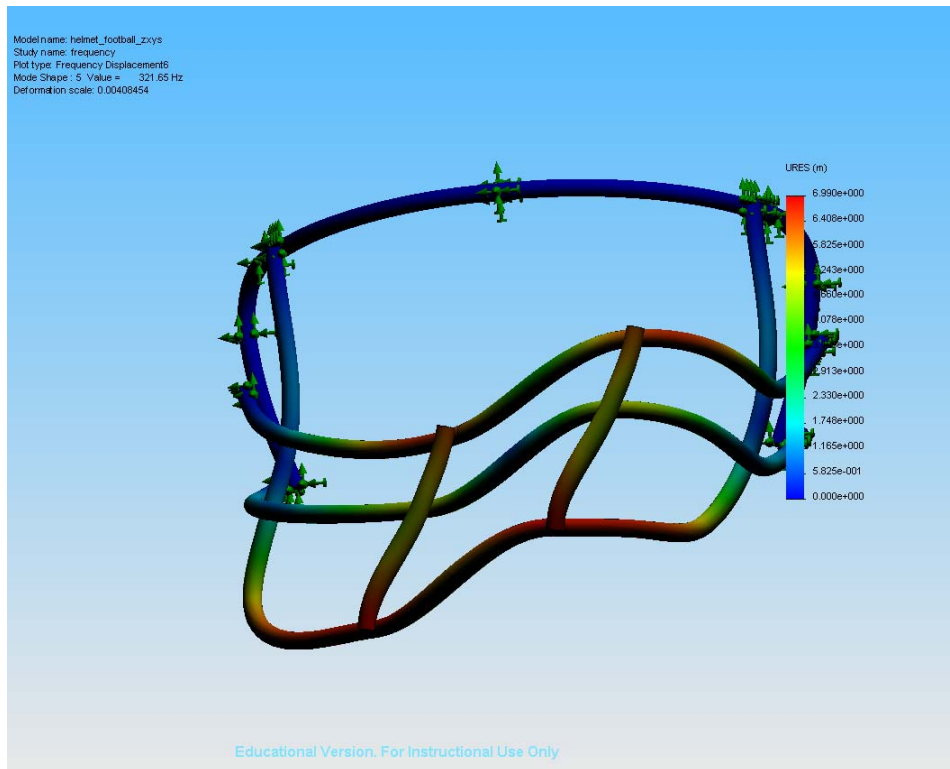
Figure 5: Frequency 5 at mesh size 0.1
