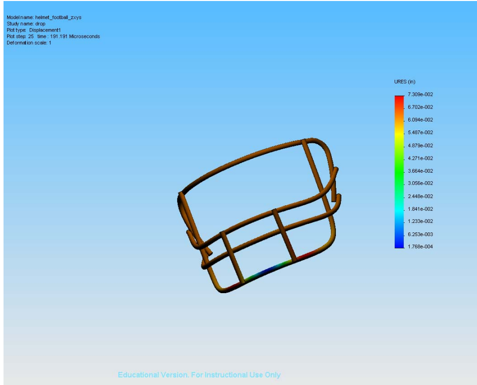
Figure 8: Displacement plot after drop test
