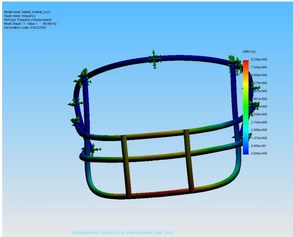
Figure 1: Modal shape & deformation at frequency 1
