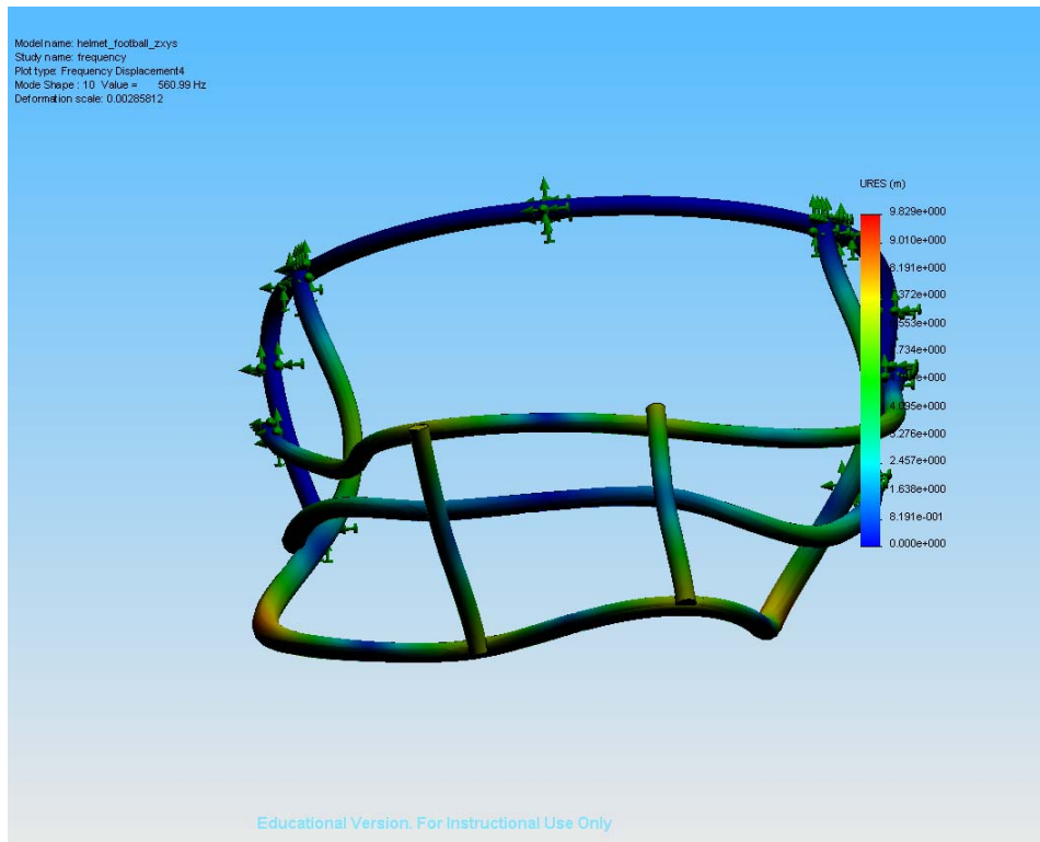
Figure 3: Modal shape & deformation at frequency 10
